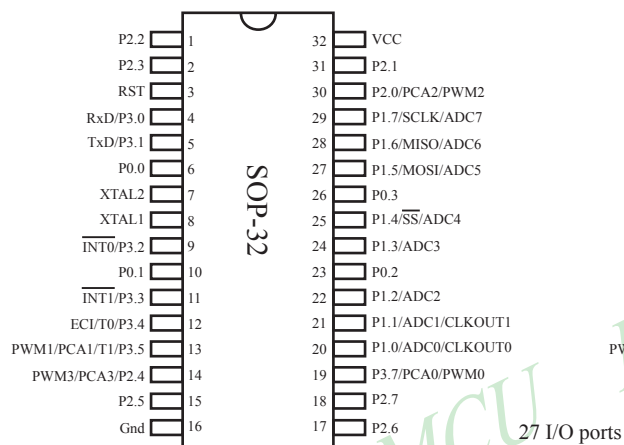
STC12C5410AD series (with A/D Converter), SOP-32
