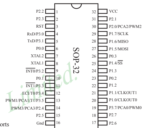
STC12C5410 series (without A/D Converter), SOP-32
