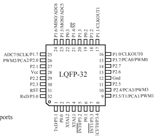
STC12C5410 series (without A/D Converter), LQFP-32
