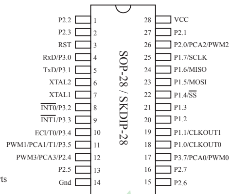
STC12C5410 series (without A/D Converter), 28-Pin
